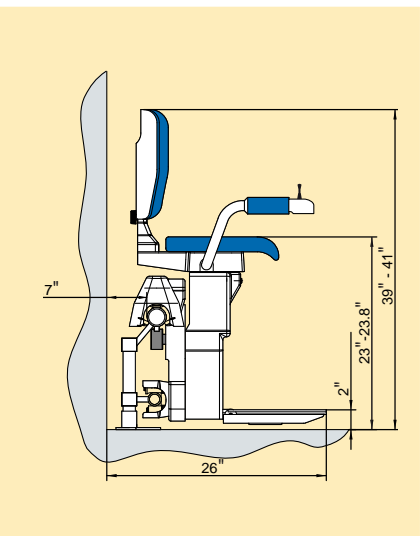
Dimensions of stairlift in unfolded park position
