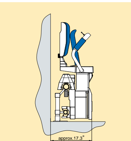
The stairlift can be folded away to only 17.3"
