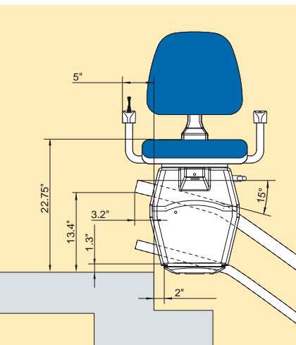
Incline finish with optional swivel seat
