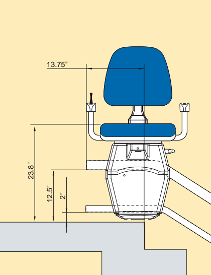
Standard horizontal finish parking position
